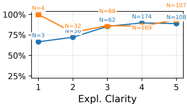
Under-reliance Mitigation Rate
